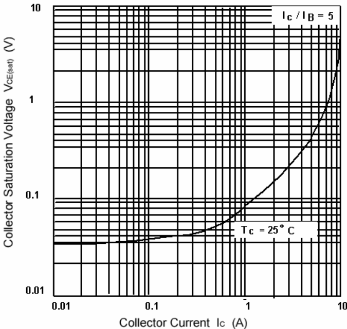
Fig.4 Collector-Emitter Saturation Voltage
