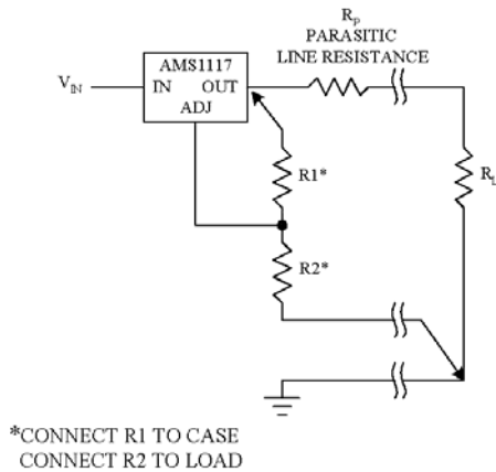
Figure 3. Connections for Best Load Regulation
