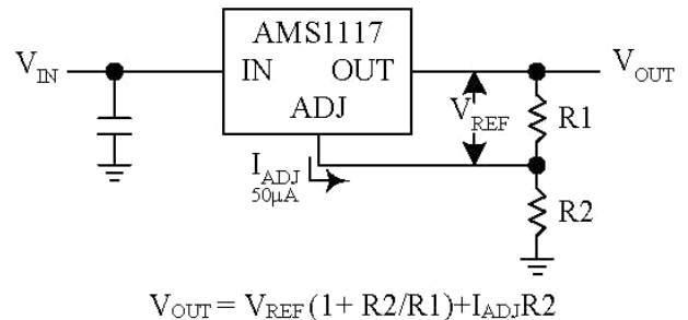
Figure 2. Basic Adjustable Regulator
