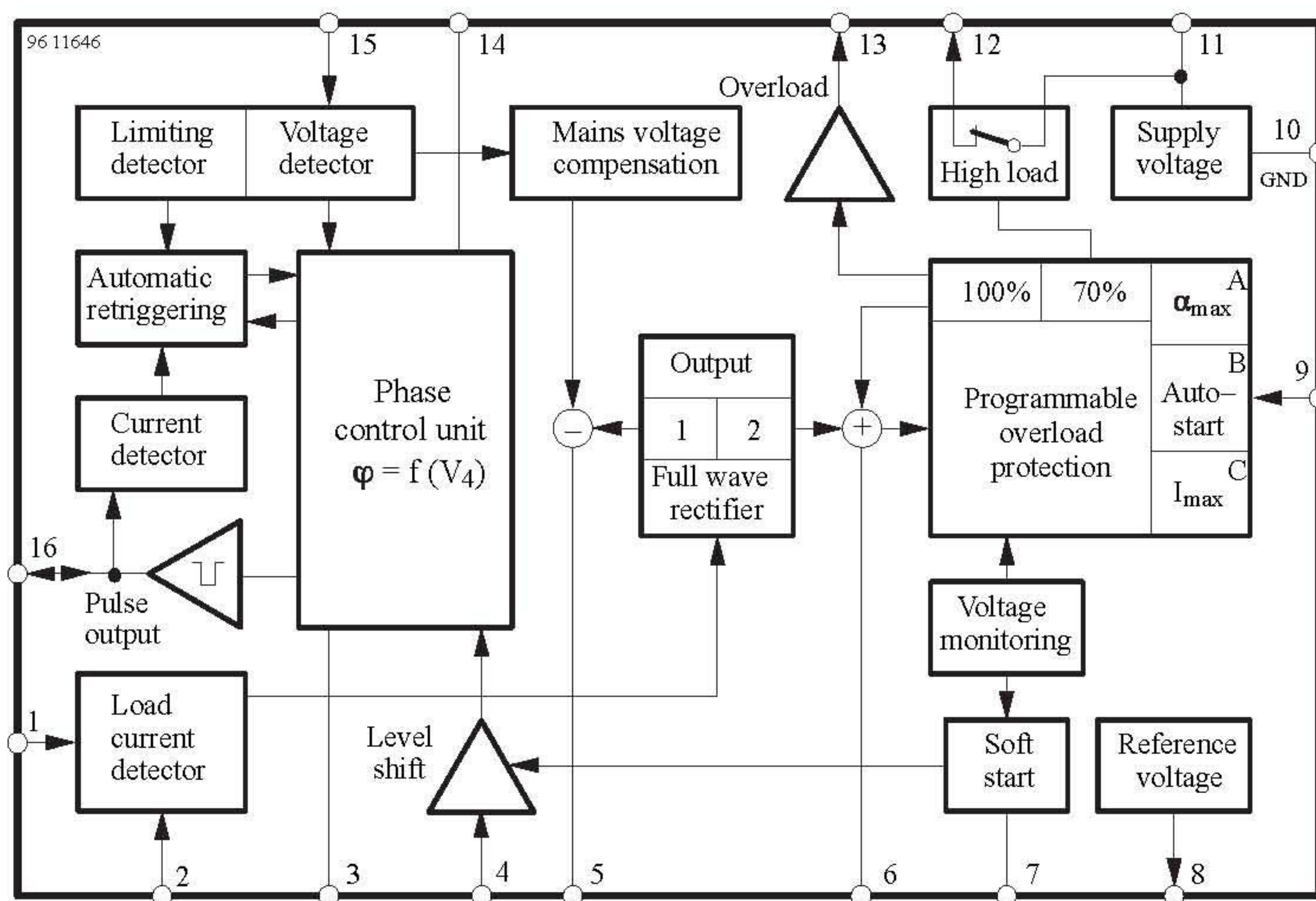
Figure 1. Block diagram
