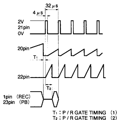
Fig. 6 P/R gate timing chart (V interval)
