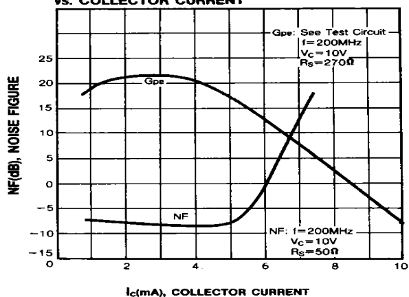
POWER GAIN AND NOISE FIGURE vs. COLLECTOR CURRENT
